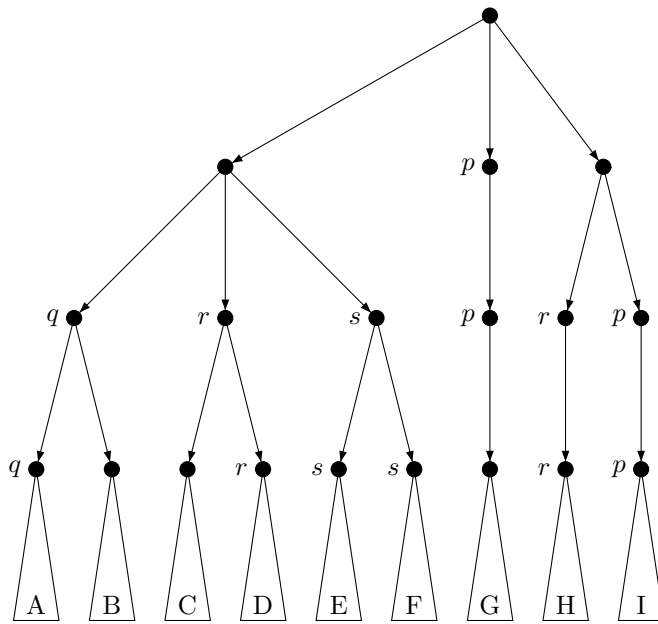
FIGURE 8. Another run with leaves on level m + 1 .
