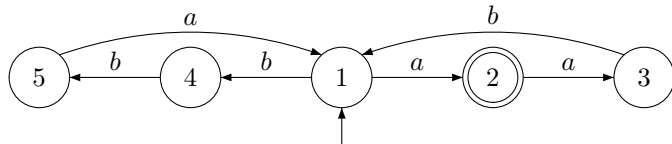
FIGURE 2. The deterministic and counter-free Büchi automaton \mathcal{A}_2
