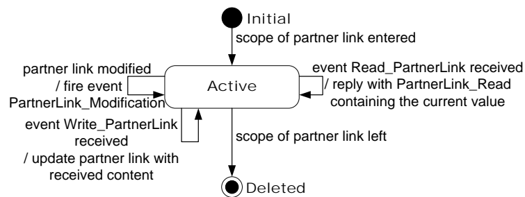
Figure 10.3: Partner Link State Chart
