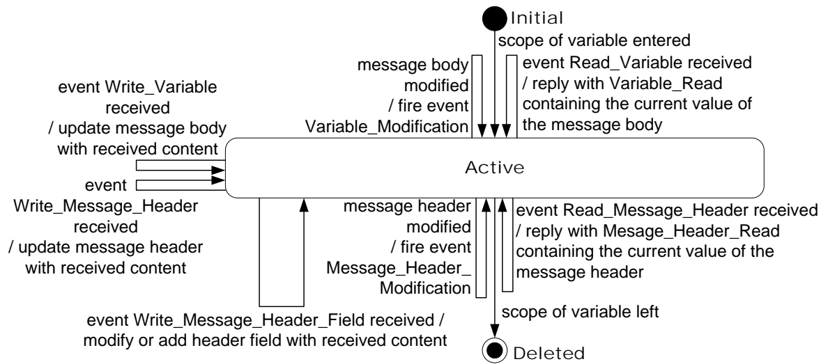
Figure 10.2: Message Variable State Chart
